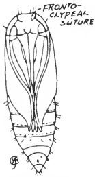
Fig. 520. Cryptotechia quercicella Clemens.
